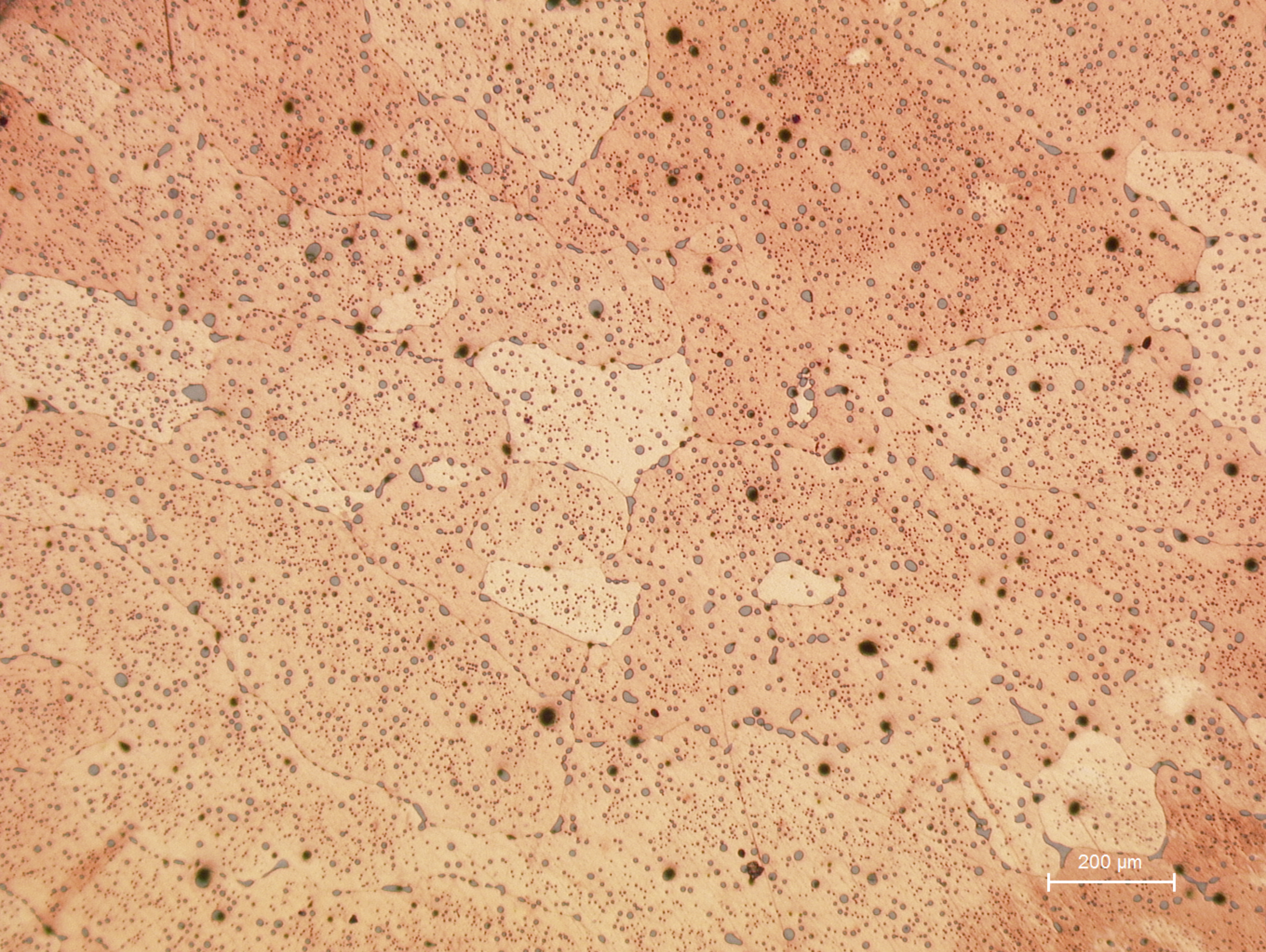
A142.1 General view of the cross section: numerous sulphide inclusions, many of them decorating the grain boundaries.
