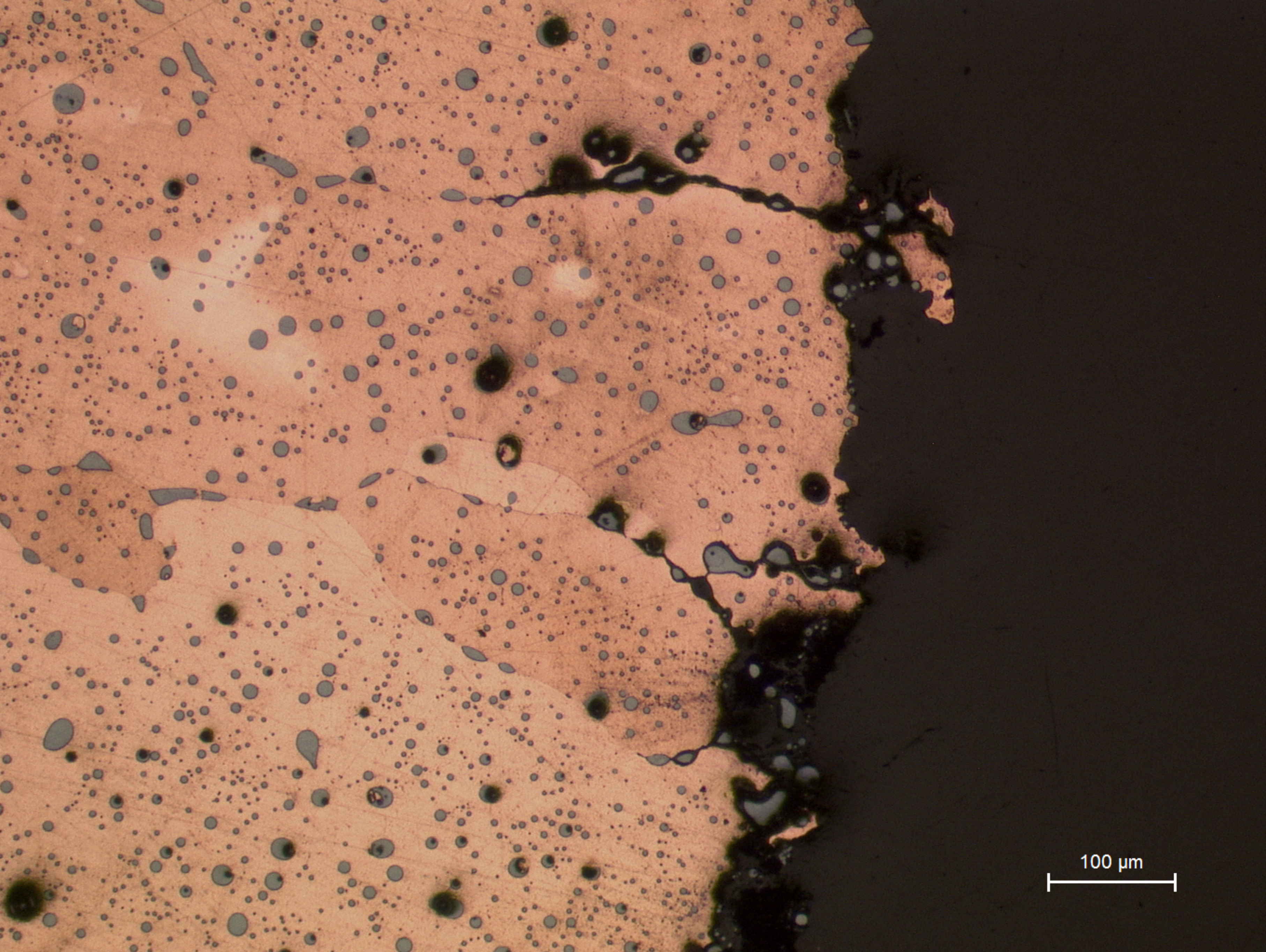
A142.2 Surface detail: corrosion penetrating intergranularly.
