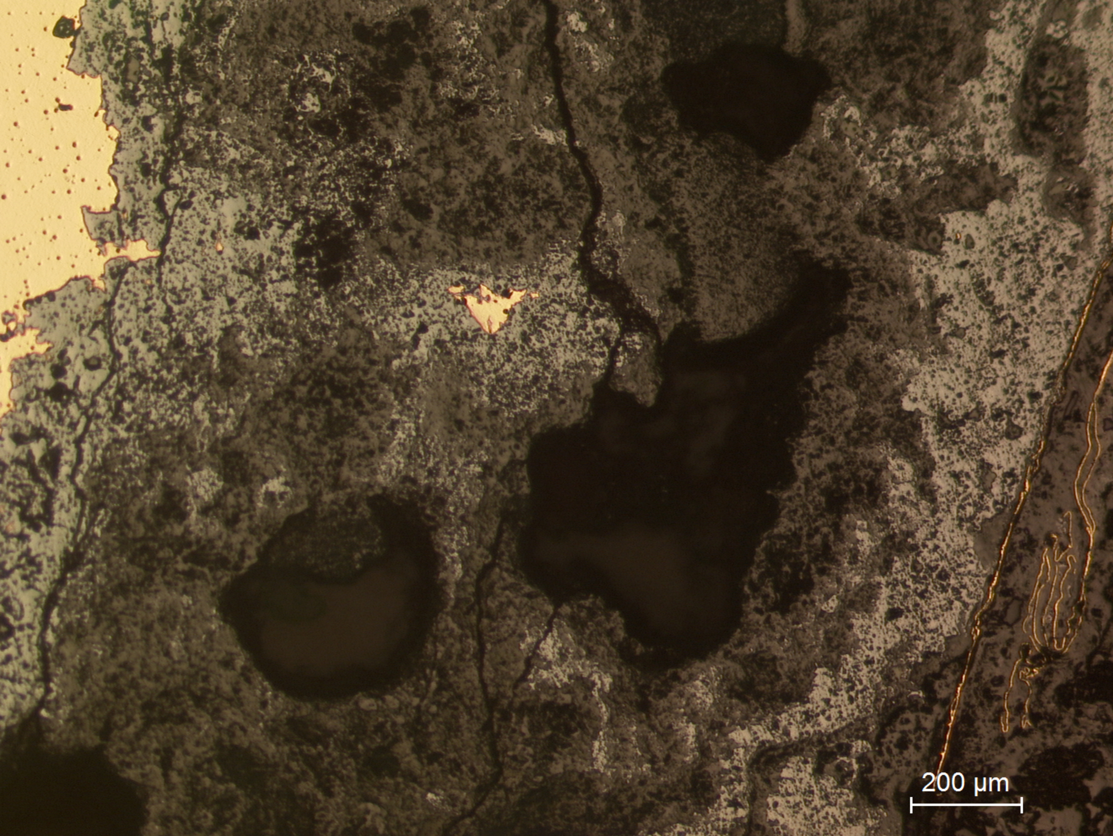
A148.2 Detail showing remains of gilding at the original surface (epidermis) in the middle of corrosion products.
