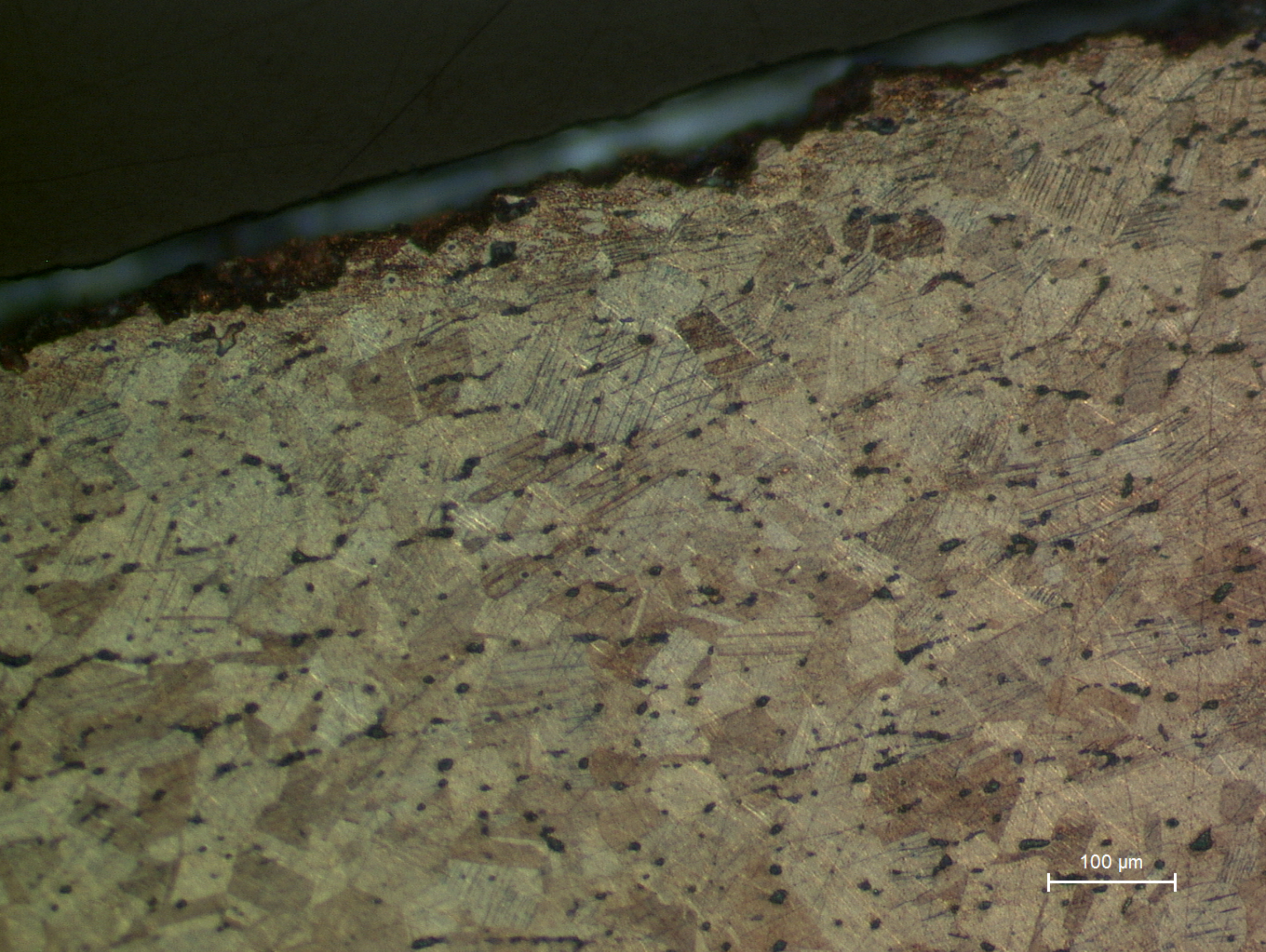
A183.2 General view showing recrystallized equiaxed grains with annealing twins; near the surface some strain lines and mechanical twins can be seen (etchant: aqueous \text{FeCl}_3 ).
