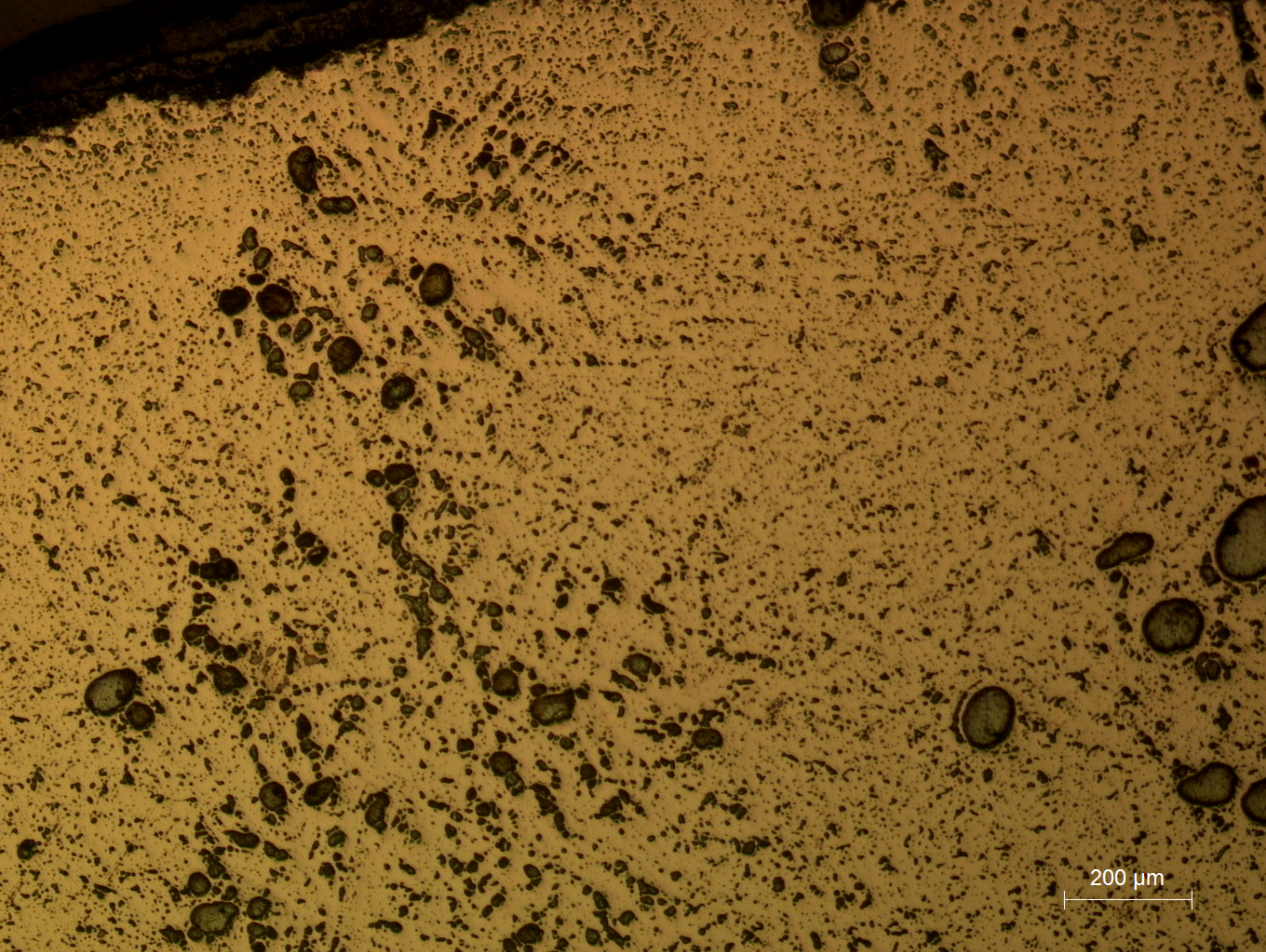
A79.1 General view: impurities heterogeneously distributed; Pb globules are clearly visible.
