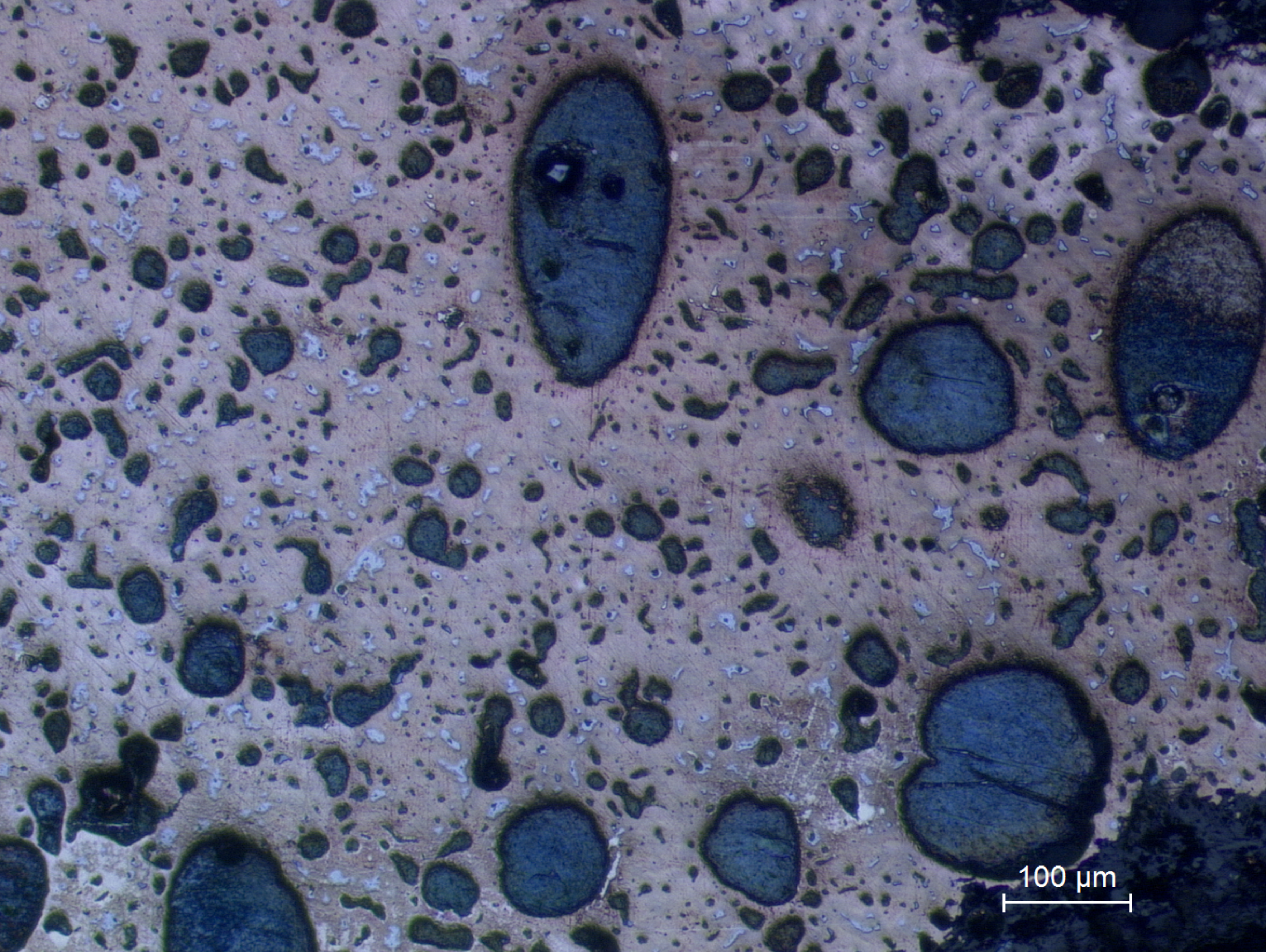
A79.2 Detail: presence of a finely divided eutectoid (white) and very large Pb particles (etchant: aqueous \text{FeCl}_3 ).
