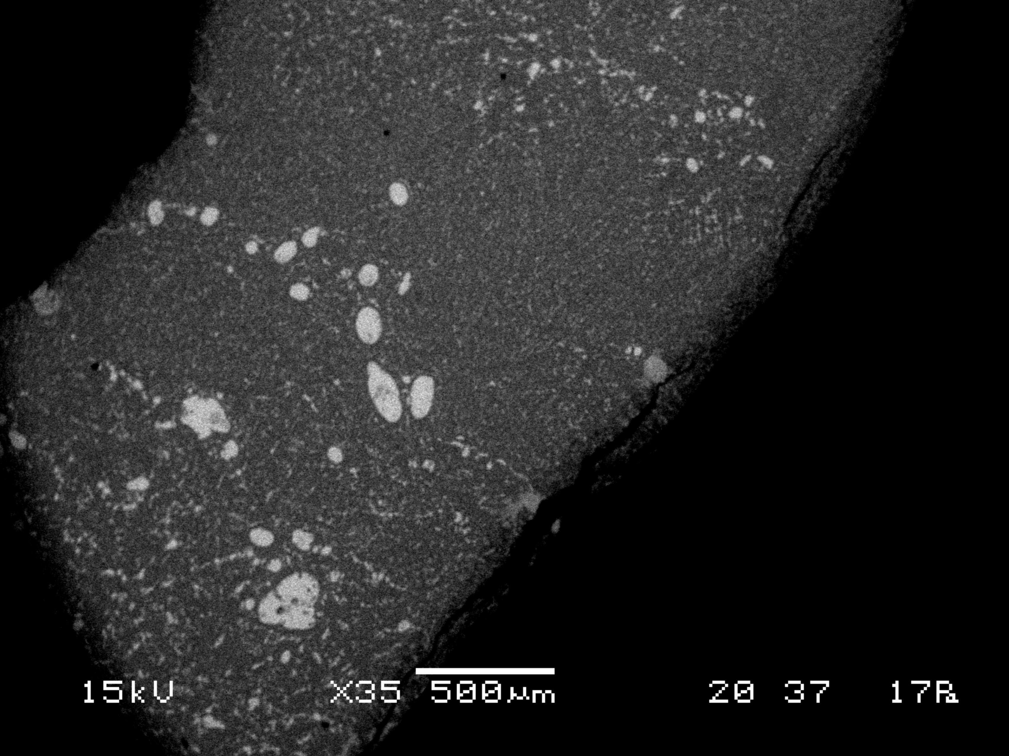
A79.3 SEM image showing the Pb particles in white (chemical contrast).
